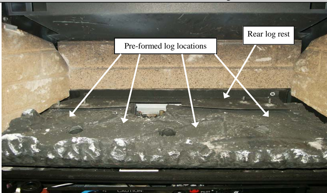
FiberFlame Burner Bed and Rear Log Rest
