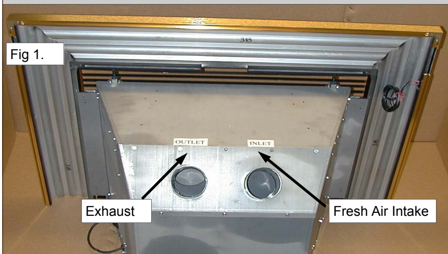
The Optima 32 showing the Exhaust and Fresh Air Intake locations. These connections are labeled for you.
