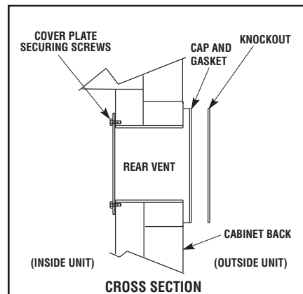
Figure 16: Rear vent seal and cover plate removal—MPD35/40/45 series models (combined top and rear vent units)
