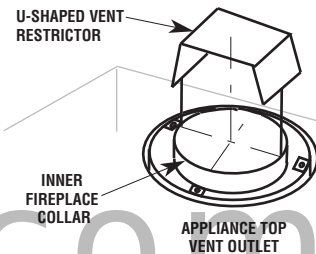
Figure 17: Vent restrictor installation—Top vent
