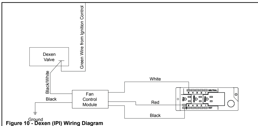
Figure 10 - Dexen (IPI) Wiring Diagram
