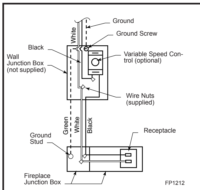
Fig. 9 SCVS wiring diagram.
