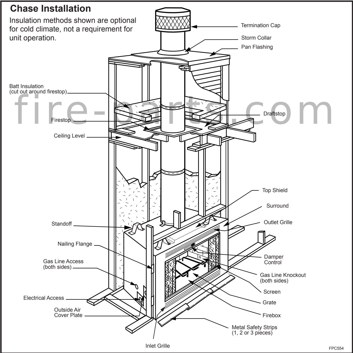
Fig. 3 Fireplace and chase parts identification.
