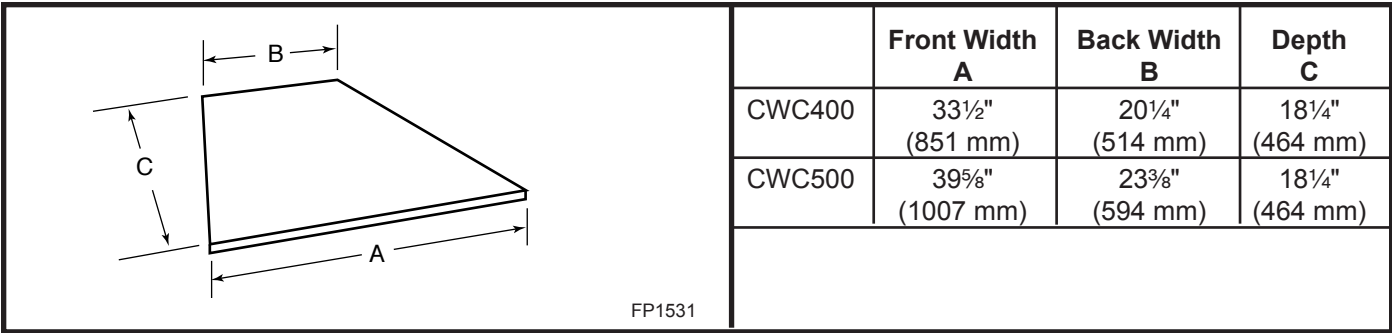
Fig. 2a Hearth dimensions.
