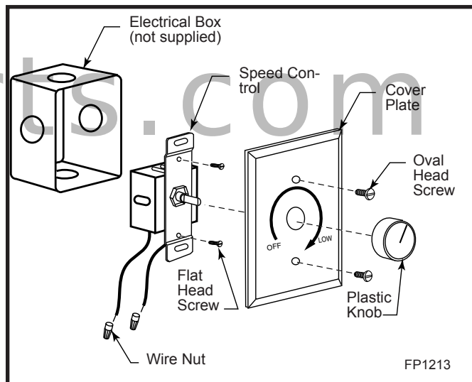
Fig. 10 Speed control mounting.
