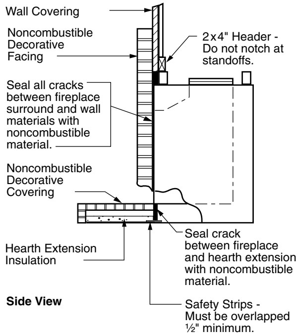
Fig. 26 Sealing gaps.
