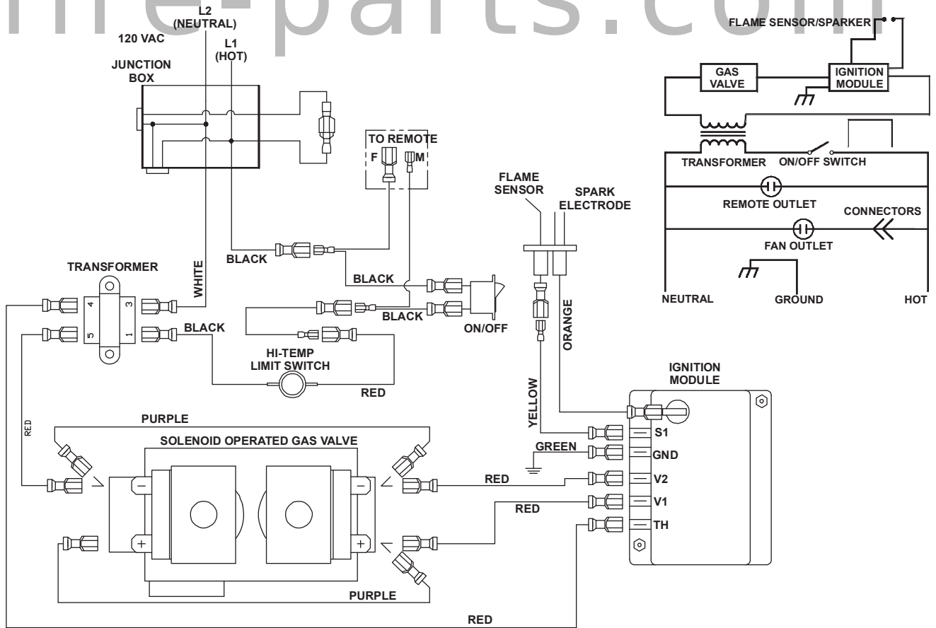
Figure 12. Direct Spark Ignition (DSI) Diagram
