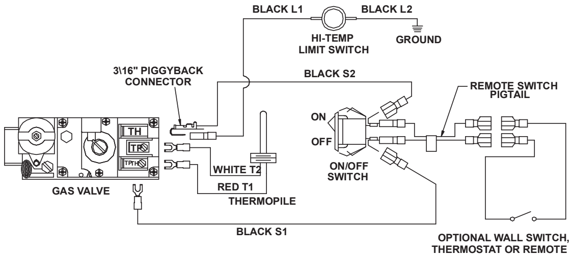
Figure 10. Standing Pilot Ignition Wiring Diagram
