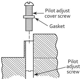
Figure 8. Pilot Gas Adjustment
