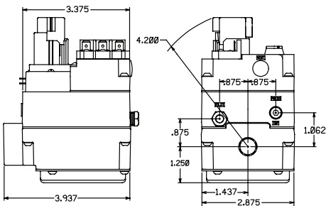
Figure 2. Valve Dimensions
