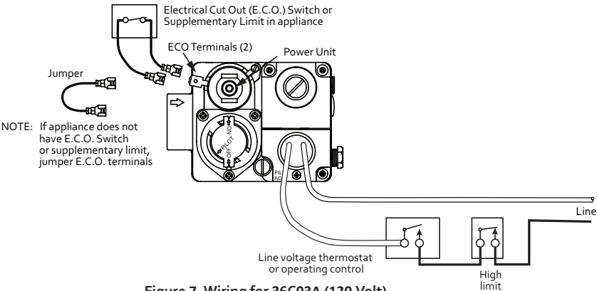
Figure 7. Wiring for 36C03A (120 Volt)
